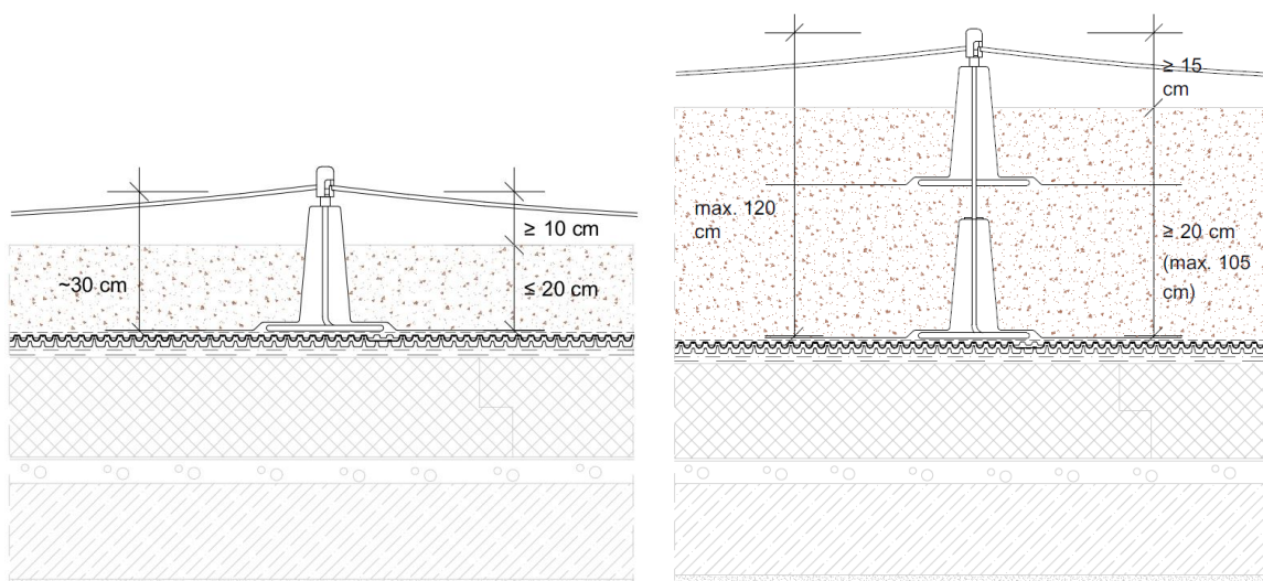
Thickness of ballast material \leq 20 cm
